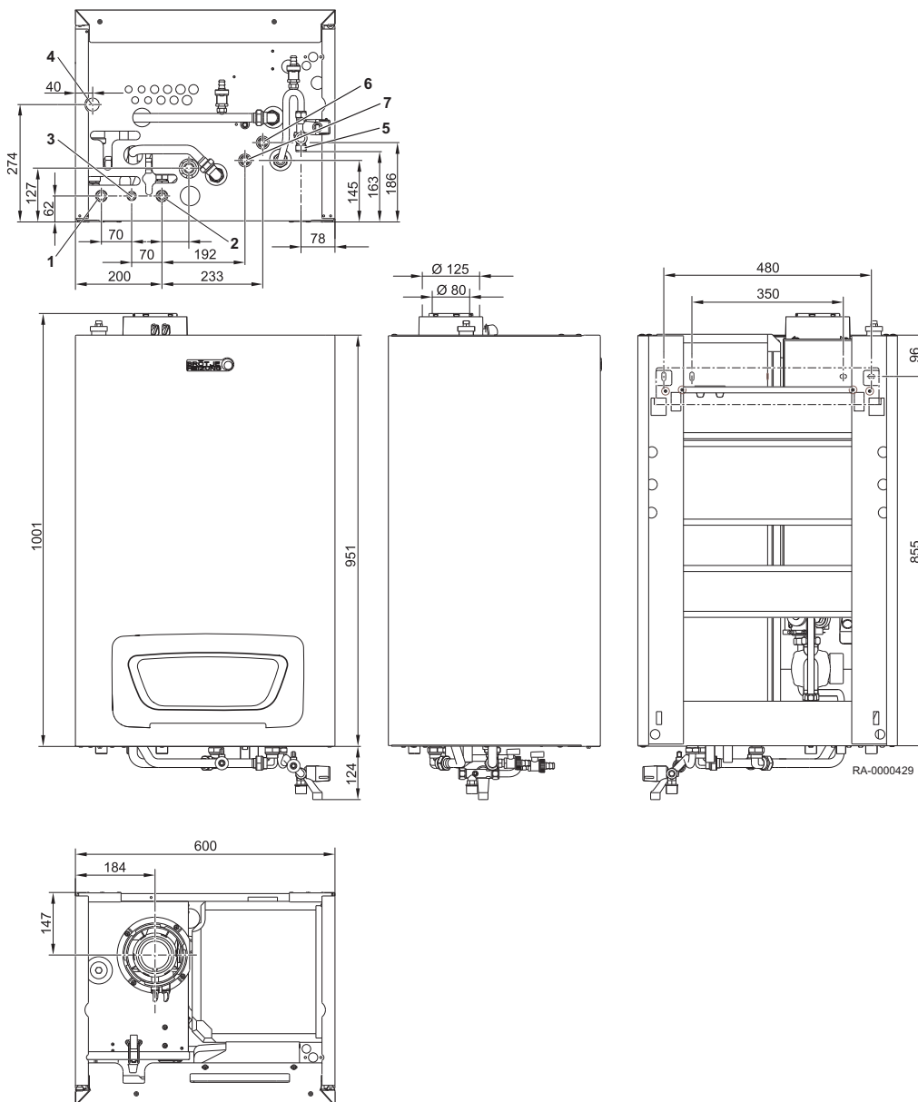
Fig.2 Dimensions et raccords WGB-K EVO
