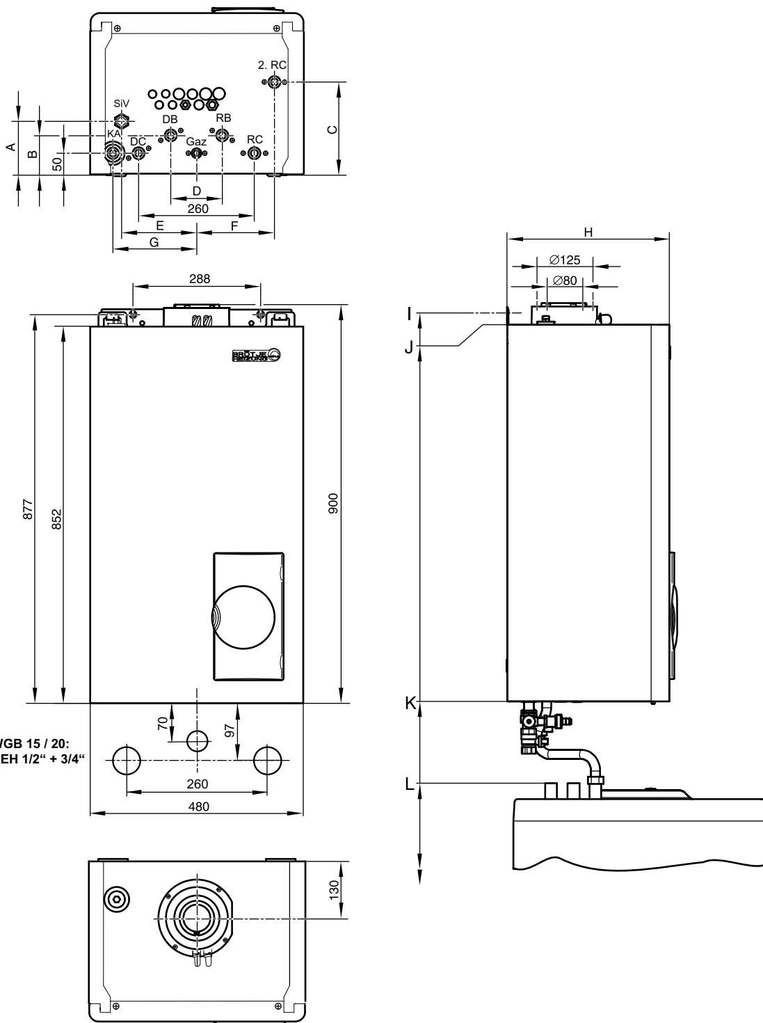
Fig 1: Dimensions et raccords
