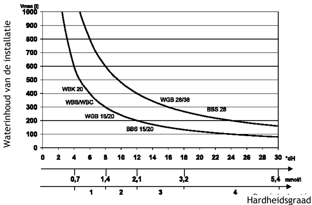
Schets2: Hydrometrisch diagram
